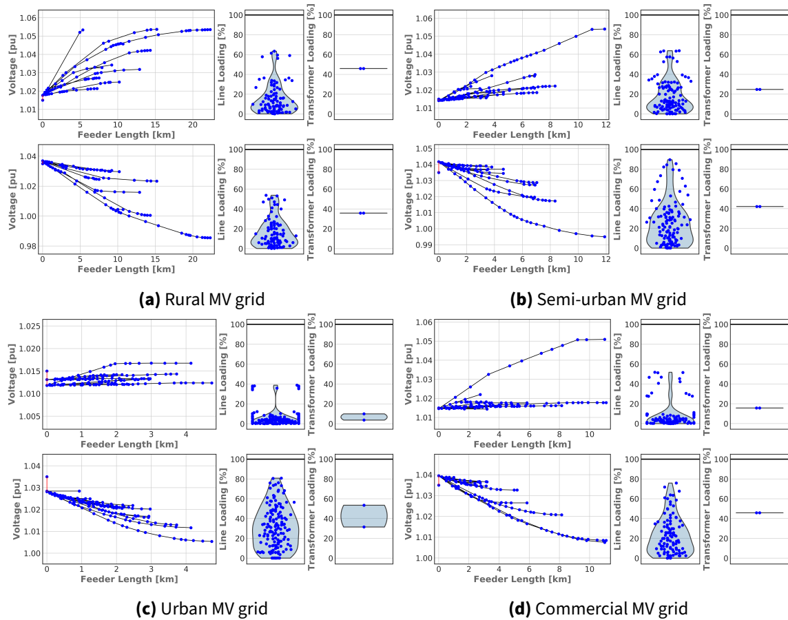
Figure 4.11: Voltage values in dependency on the distance to the HV/MV transformer station as well as line and transformer loadings for the study cases LW (top) and hL (bottom)
