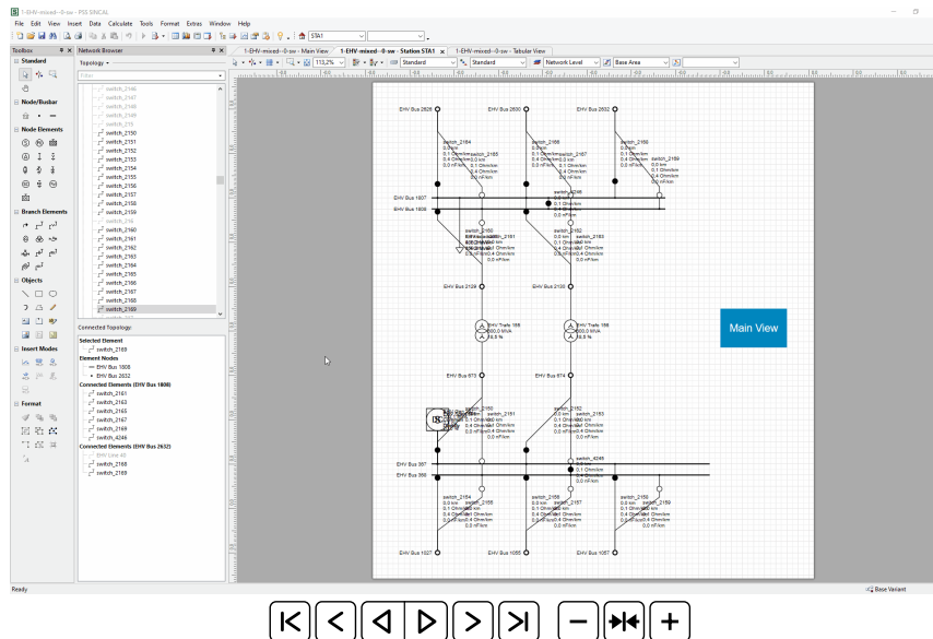
Figure C.4: Demonstration of how to edit the substation view
