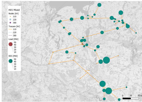
(a) Regenerative Power Plants in HV1
