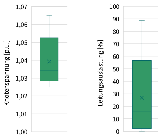
Figure 5.3: Results of the basic power flow calculation for the grid “1-HV-urban--0-sw” in case of load “IW” depicted by boxplots
