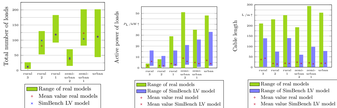
Figure 4.13: Comparison of real network data with SimBench LV networks with regard to number of loads (left), active load power (center) and cable lengths (right)
