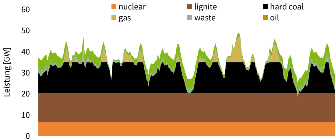
Figure 3.4: Power plant dispatch for an exemplary week
