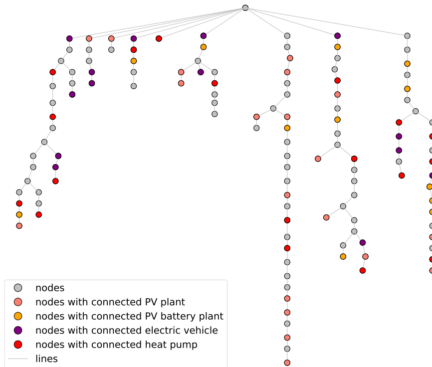
Figure 4.21: Picture of the LV grid LV3 in scenario 2 for the year 2034
