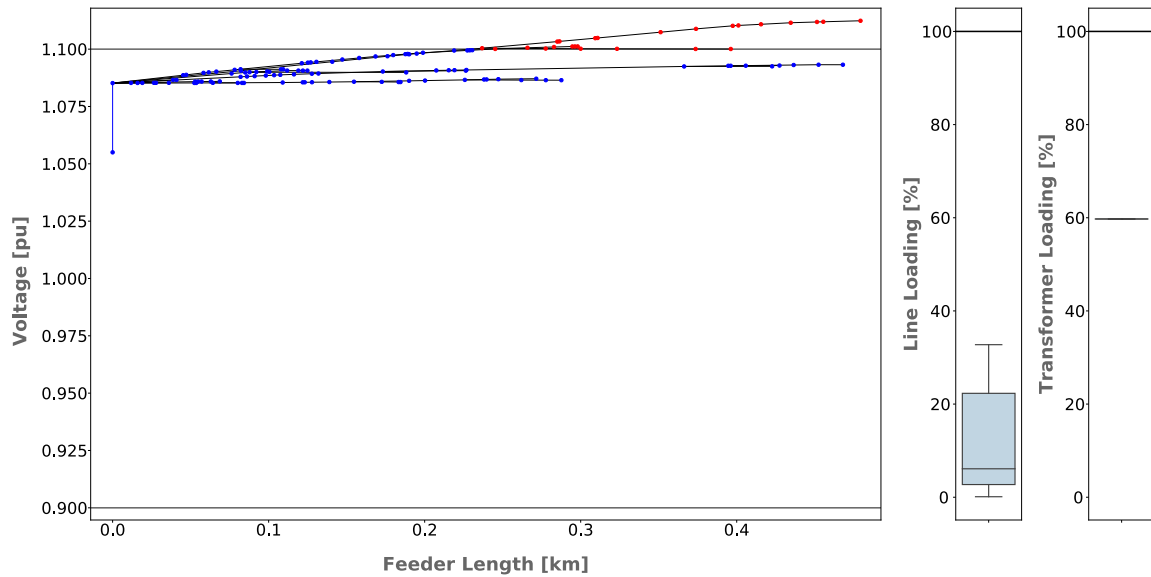
Figure 4.23: Violations detected in LV grid LV3 in scenario 1
