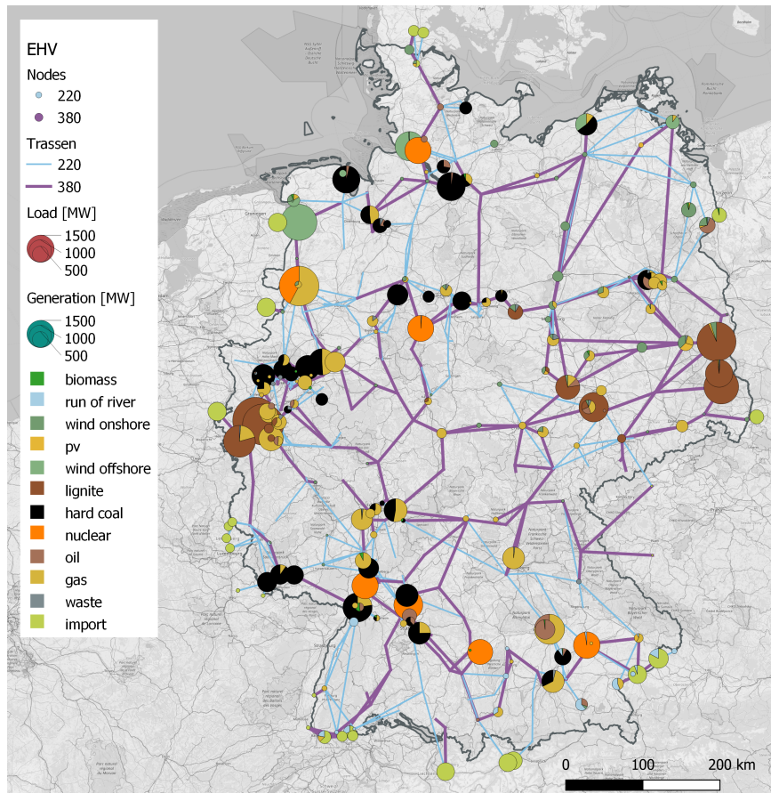
Figure 4.3: Geographical Distribution of Renewable Energy Power Plants and Conventional Power Plants
