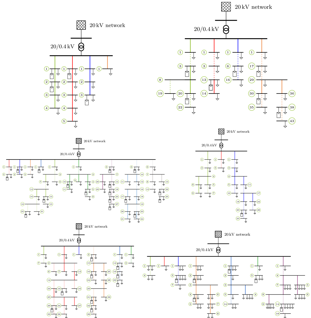
Figure 4.12: Schematic representation of the LV networks (from top left to bottom right): three rural networks, two suburban networks and one urban network.
