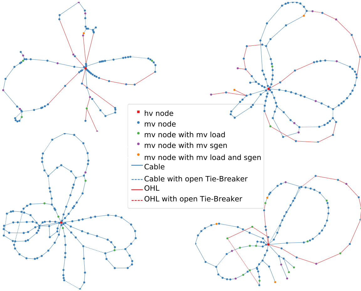
Figure 4.9: Plot of MV grids: rural (top left), semi-urban (top right), urban (bottom left) and commercial (bottom right)
