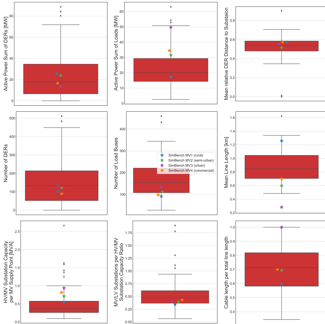
Figure 4.10: Comparison of grid parameters of SimBench MV grids and real grids
