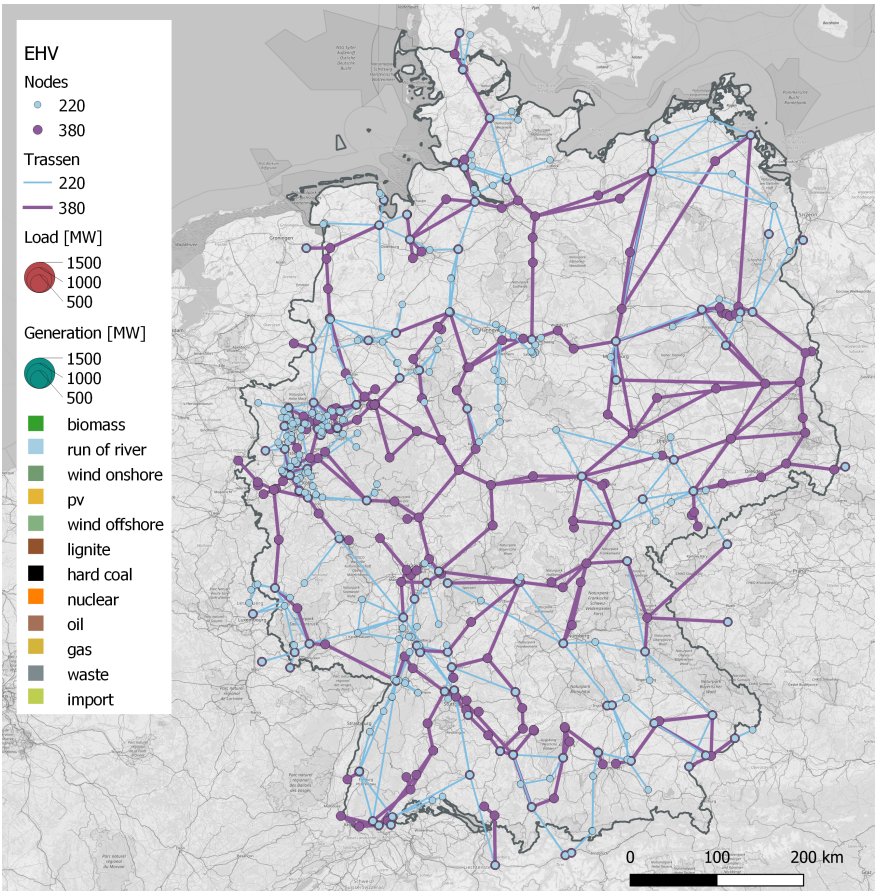
Figure 4.1: Topology of the EHV network
