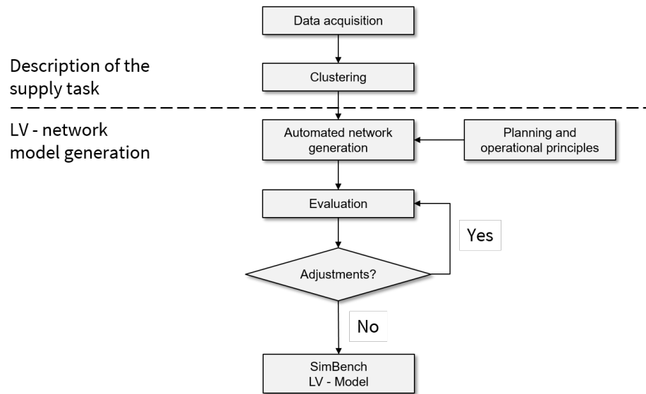
Figure 3.10: Methodology for LV network model generation
