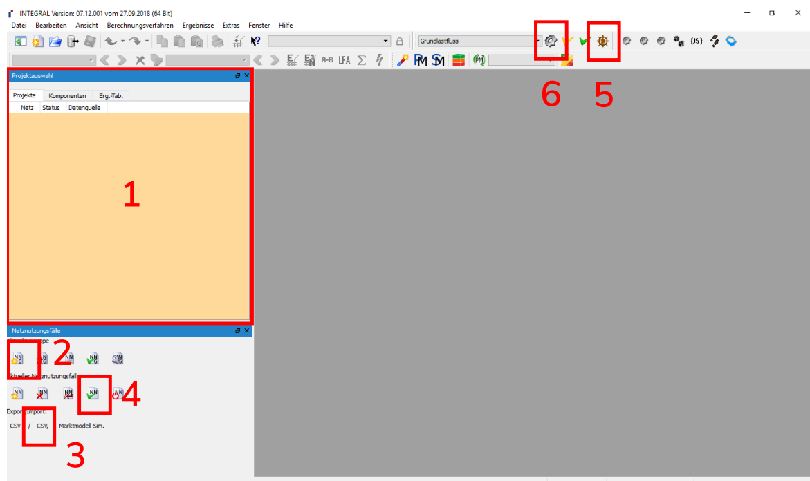
Figure C.6: INTEGRAL User Interface
