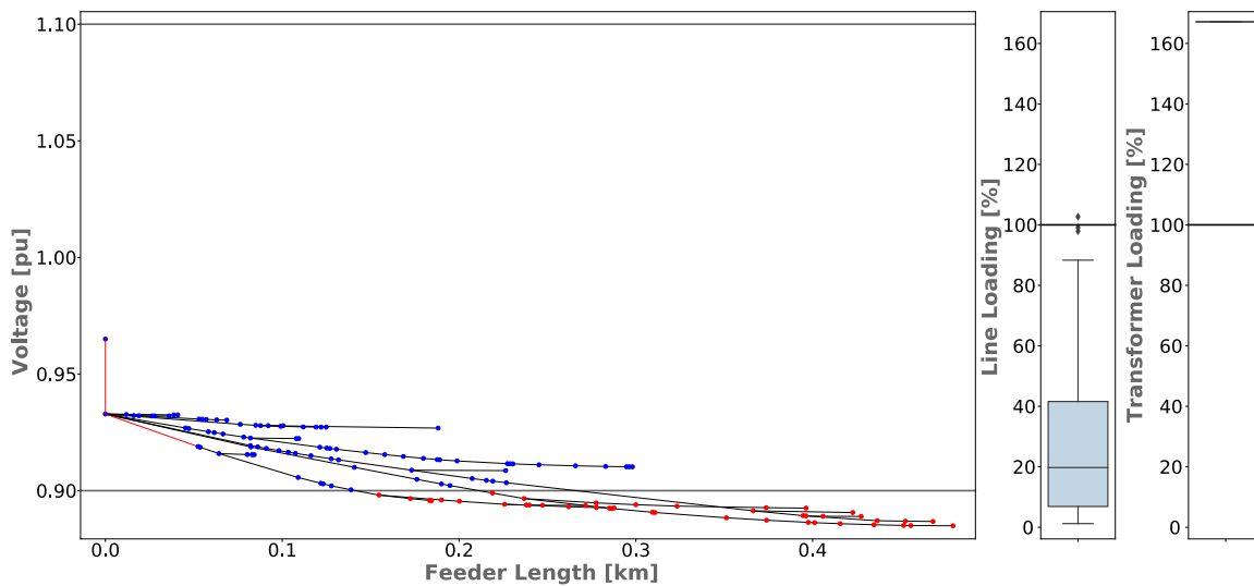
Figure 4.24: Violations detected in LV grid LV3 in scenario 2
