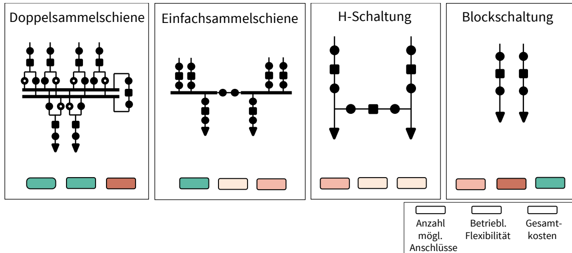
Figure 3.9: Station concepts in the HV level
