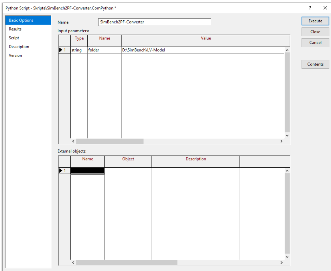
Figure C.5: Structure of the Python Command Object in PowerFactory
