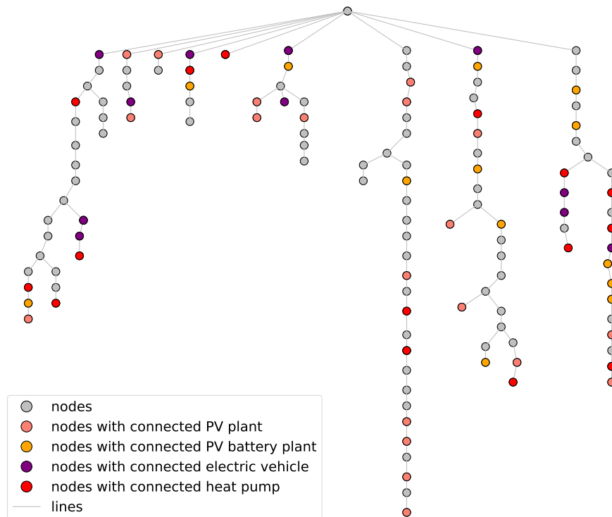
Figure 4.20: Picture of the LV grid LV3 in scenario 1 for the year 2024
