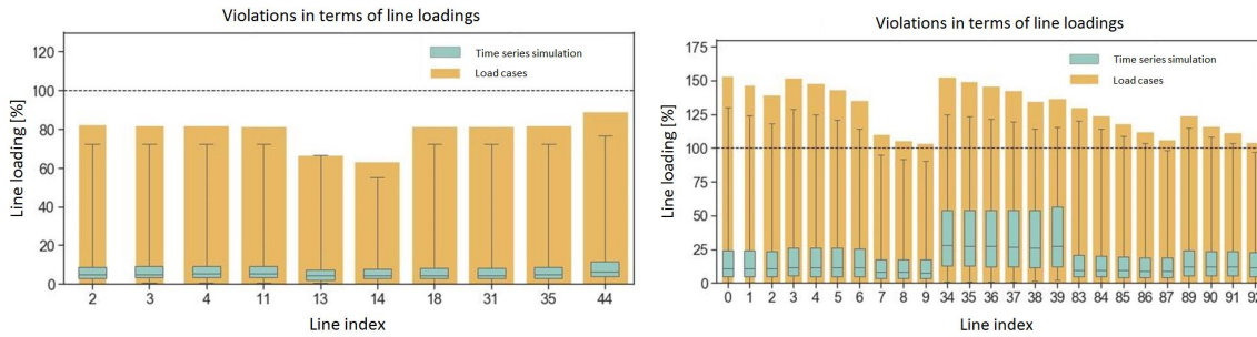
Figure 5.5: Comparison of the maximum line loadings based on all defined calculation cases (except n-1) and the annual time series simulations exemplary for the urban LV grid (seen left) and suburban MV grid (seen right) in case of scenario 1
