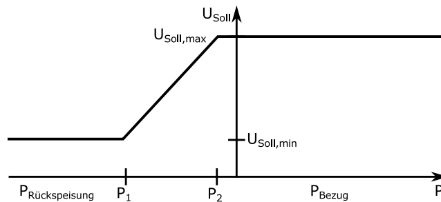
Figure 5.2: Characteristic curve for a simple, exemplary voltage setpoint control of HV/MV transformer tapchangers as a function of the load case
