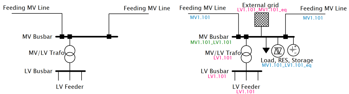
Figure 4.29: Principle of a MV/LV connection (left) including all equivalent elements and “subnet” parameters (right)
