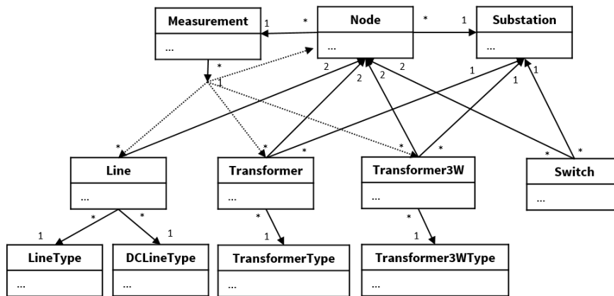
Figure 4.31: External relations of the branch elements of the SimBench CSV format
