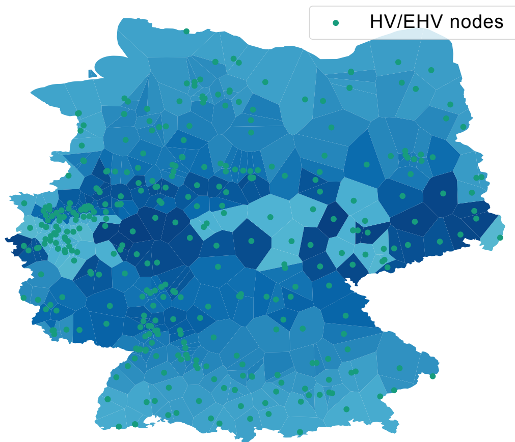
Figure 3.15: Voronoi polygons and the corresponding HV/EHV nodes
