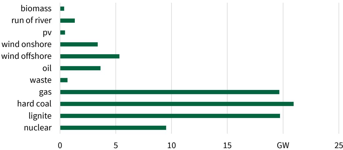
Figure 4.2: Installed power plant capacity in the EHV grid per technology
