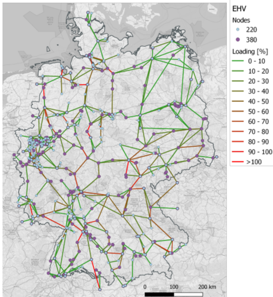
Figure 4.4: Exemplary power flow result for one hour
