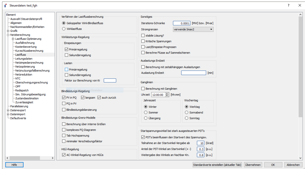
Figure 5.4: Control data in INTEGRAL
