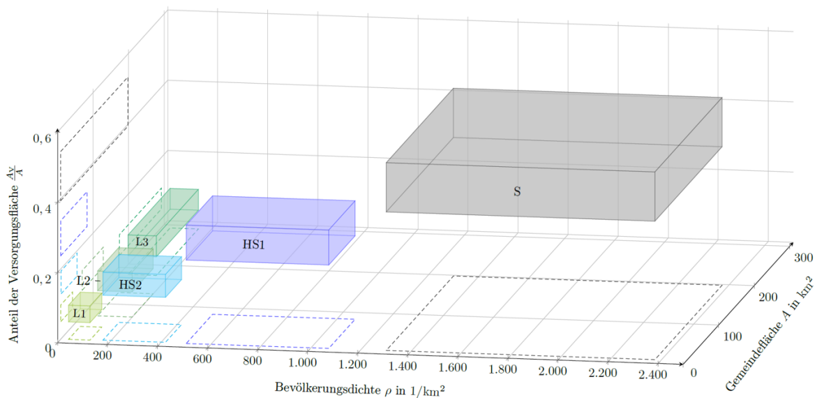
Figure 3.11: Classification result of the LV supply tasks
