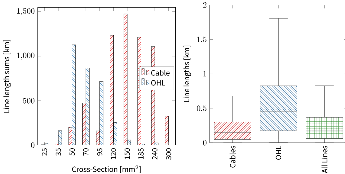
Figure 3.2: Example results of data analysis: cross-section distribution (left) and line length boxplots (right) by line type in real MV grids
