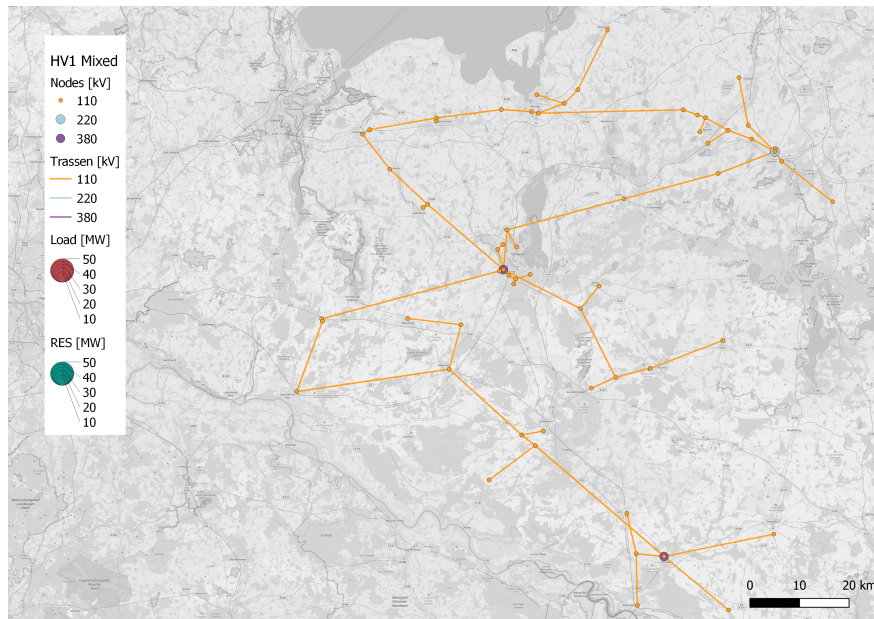
Figure 4.5: Representation of the predominantly rural HV network
