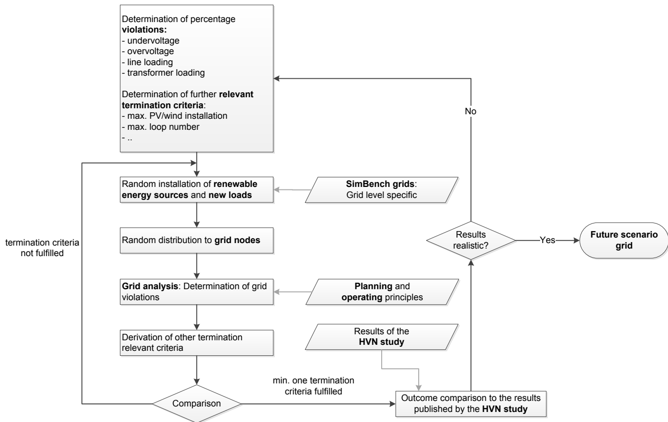
Figure 3.17: Flowchart showing the generation of the future scenarios
