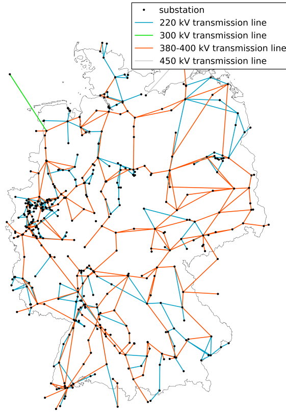
Figure 3.3: Grid model SciGrid
