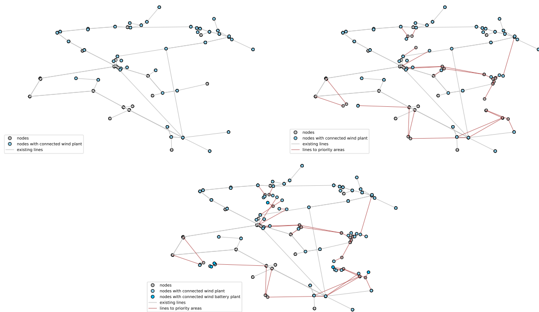
Figure 4.27: Picture of the mixedHV grid for the different scenarios (0: top left, 1: top right, 2: bottom)
