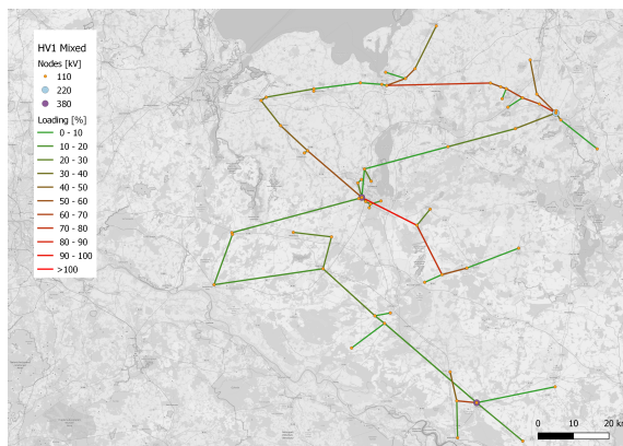
(a) HV1 grid
