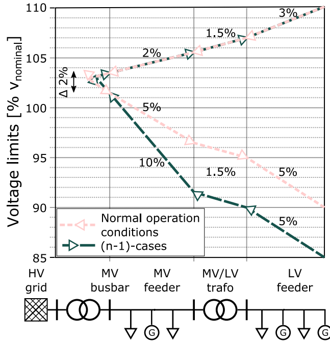
Figure 5.1: Voltage limits of MV and LV level depending on the study case
