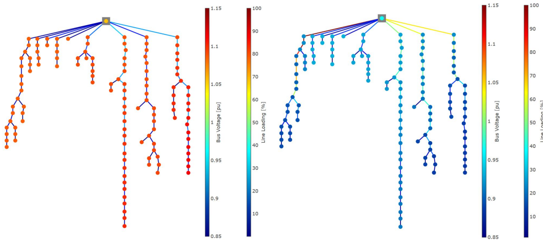
Figure 4.22: Picture of the LV grid LV3 with calculated bus voltages and line loadings displayed as heat map for scenario 1 (see left) und 2 (see right)
